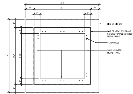
SECTIONAL FRONT ELEVATION
