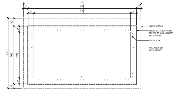
03 - FRONT ELEVATION VERTICAL
