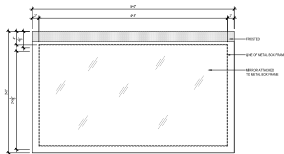
02 - FRONT ELEVATION HORIZONTAL
